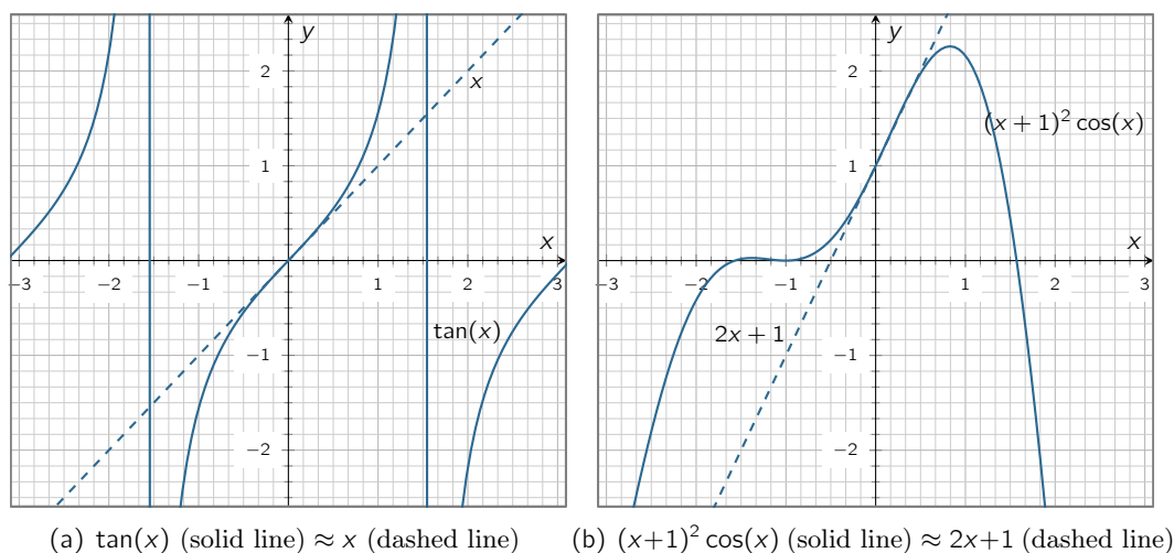
Figure 3.3: Graphical examples of the linearisation of mathematical functions around x = 0 .
