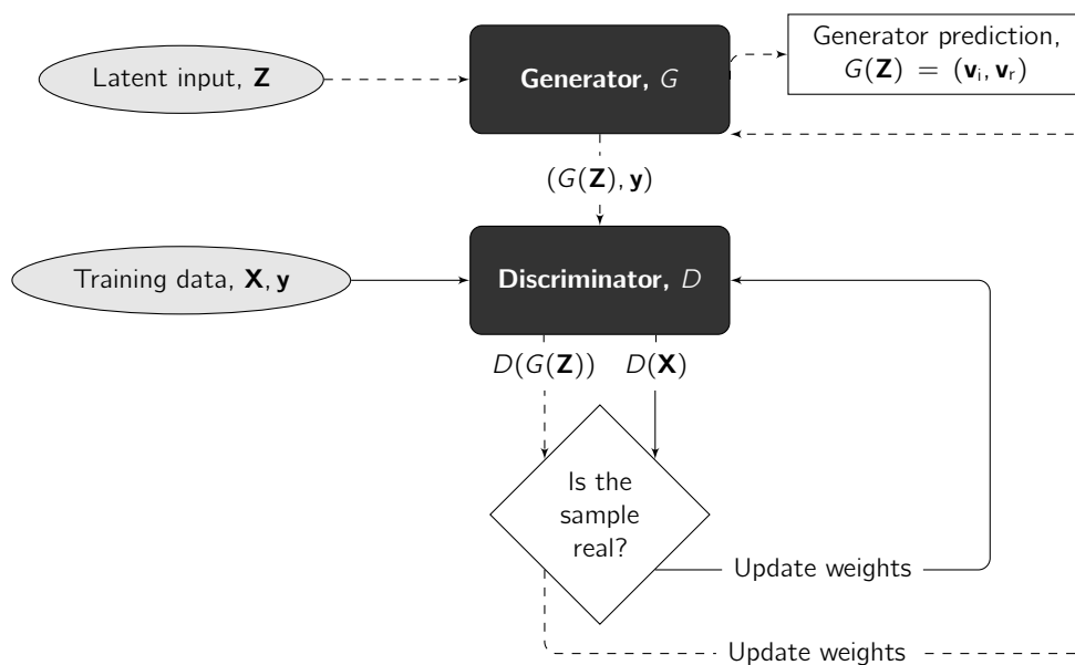
Figure 3.4: Flowchart of processes for the discriminator and generator in the GAN, where the solid line represents discriminator training, and the dashed line represents generator training.
