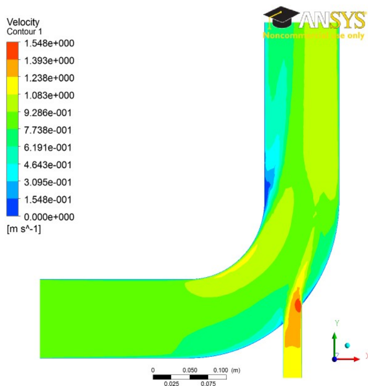
Figure 5.1: Velocity distribution on the mid-plane for an inlet velocity for case 1.
